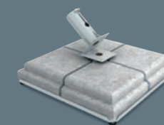
Base in ferro 90 x 90 cm e set 4 pesi in cemento Iron base 90 x 90 cm and 4 cement weights
